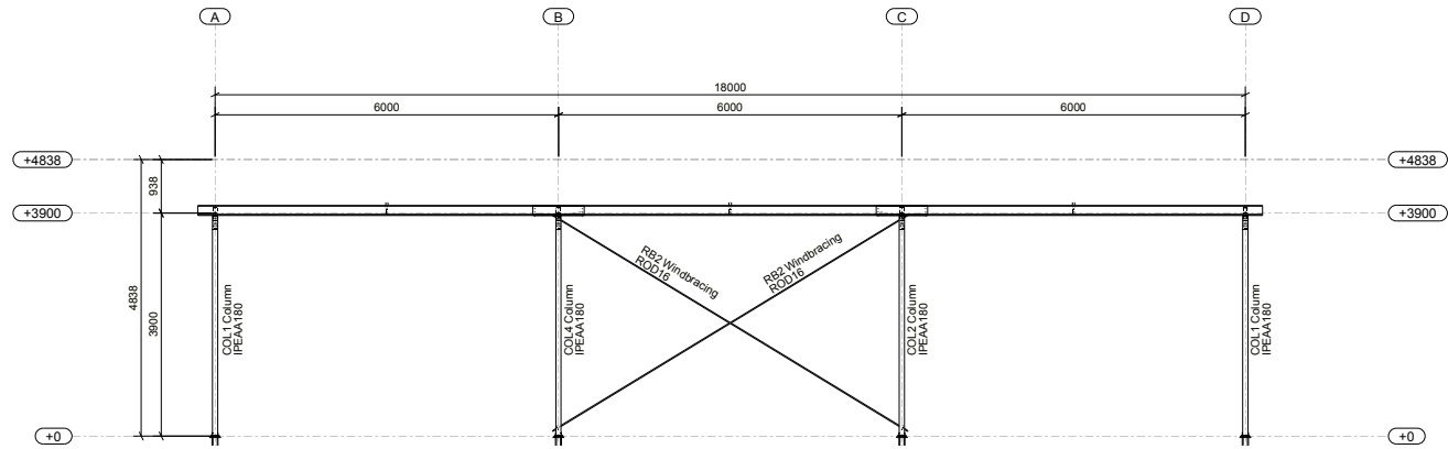
Northern Elevation (Open)
